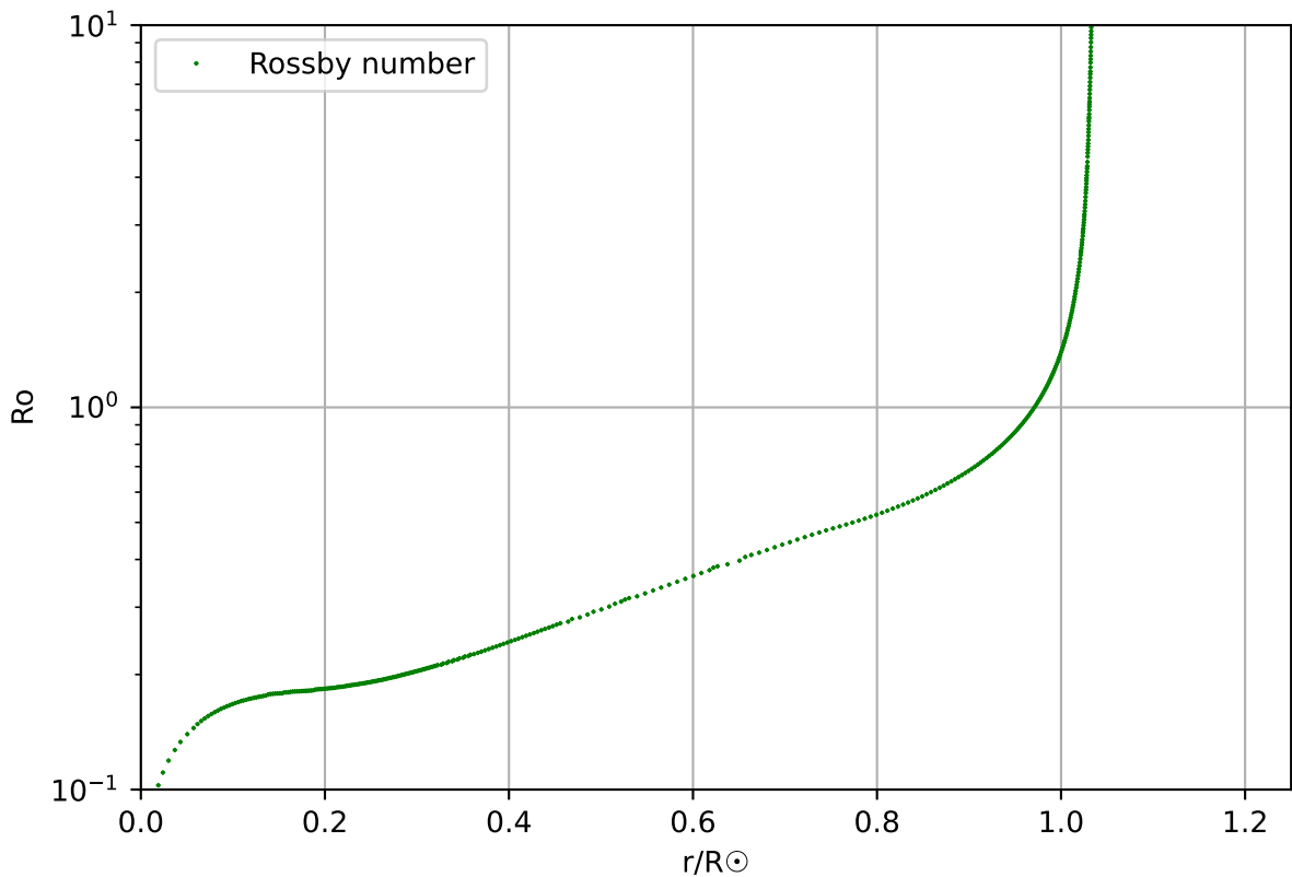
Rossby number, profile 152, age 5.8 \times 10^9
